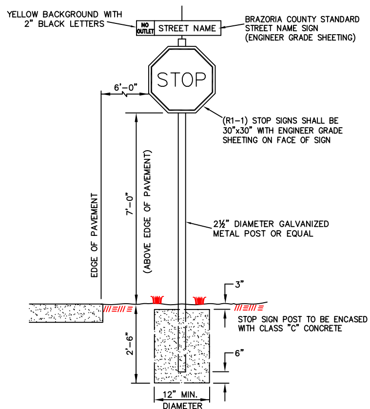
SIGN MOUNT
